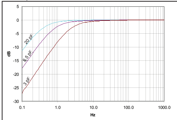
Fig. 3 Typical low-frequency response of Type 26AL for 1/2 (20 pF), 1/4 (6.5 pF) and 1/8 (3 pF) microphones
